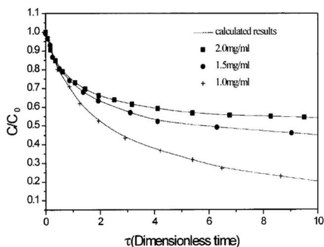
Fig. 2. The adsorption profile for BSA by the modified film and pore diffusion model at varied initial concentrations.
